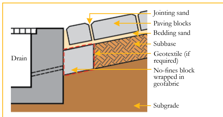
Figure 3 a – No fines block in subbase layer
