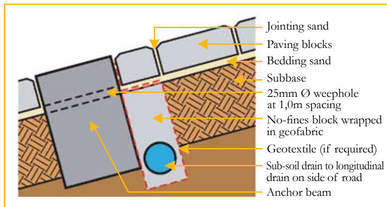
Figure 3 b – Subsoil drain drawing bedding sand water to side drain
