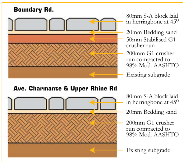
Figure 6 -Pavement layers of Cape Town roads under review
