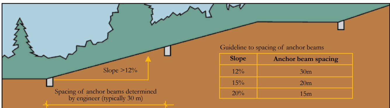
Figure 2 – Spacing of anchor beams
