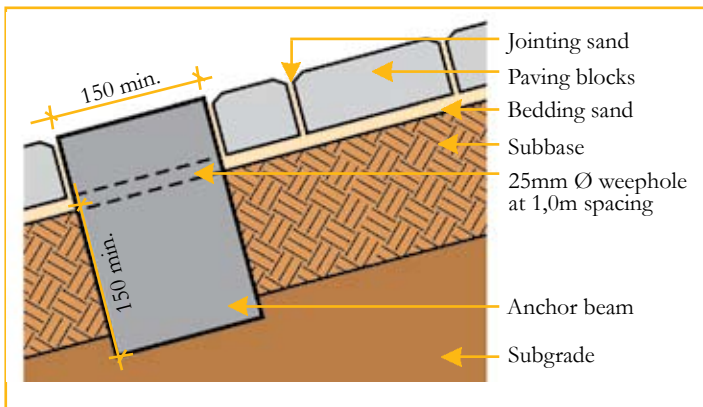
Figure 1 – Typical section through anchor beam showing dimensions
