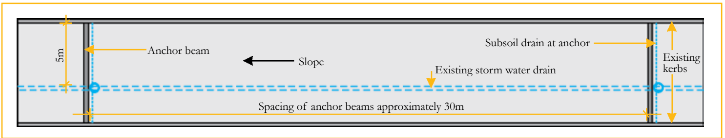
Figure 5 – Plan view of Boundary Road, Greenpoint
