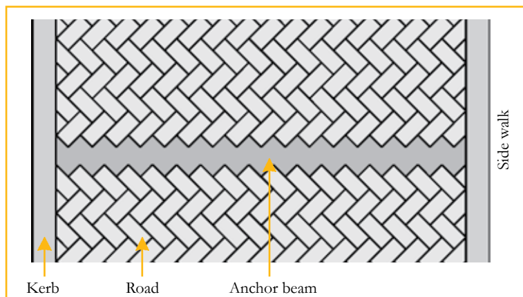
Figure 4 – Herringbone 45° to the kerbing.
